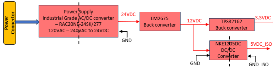
Power supply scheme SIB H Board
