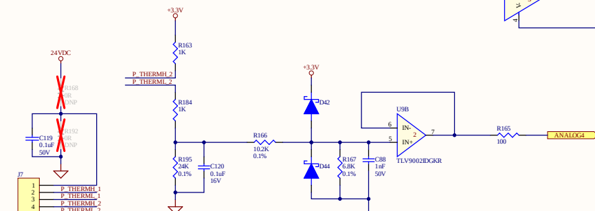
ANALOG INPUTS THERMISTOR - 2
