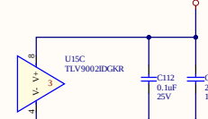
ANALOG INPUTS THERMISTOR - 3
