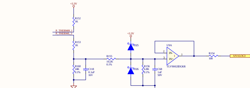
ANALOG INPUTS THERMISTOR - 1
